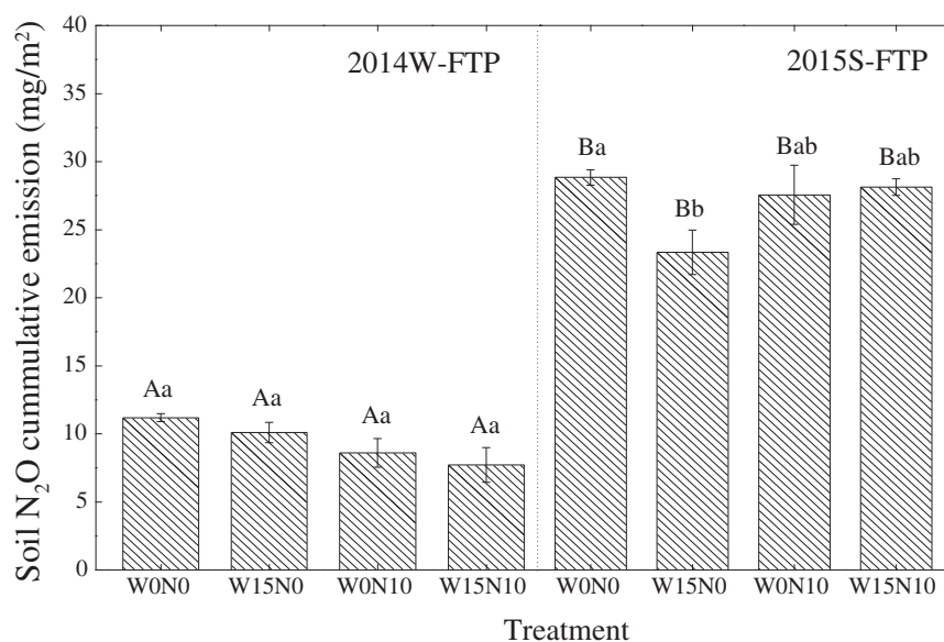
Fig. 7 – Cumulative N 2 O emissions of the different treatments. Error bars indicate the standard errors of the mean ( n = 3 ). Bars with different small letters denote treatments of the same freeze-thawing period differ significantly at p < 0.05 , bars with different capital letters denote 2014W-FTP and 2015S-FTP of the same treatment differ significantly at p < 0.05 .
