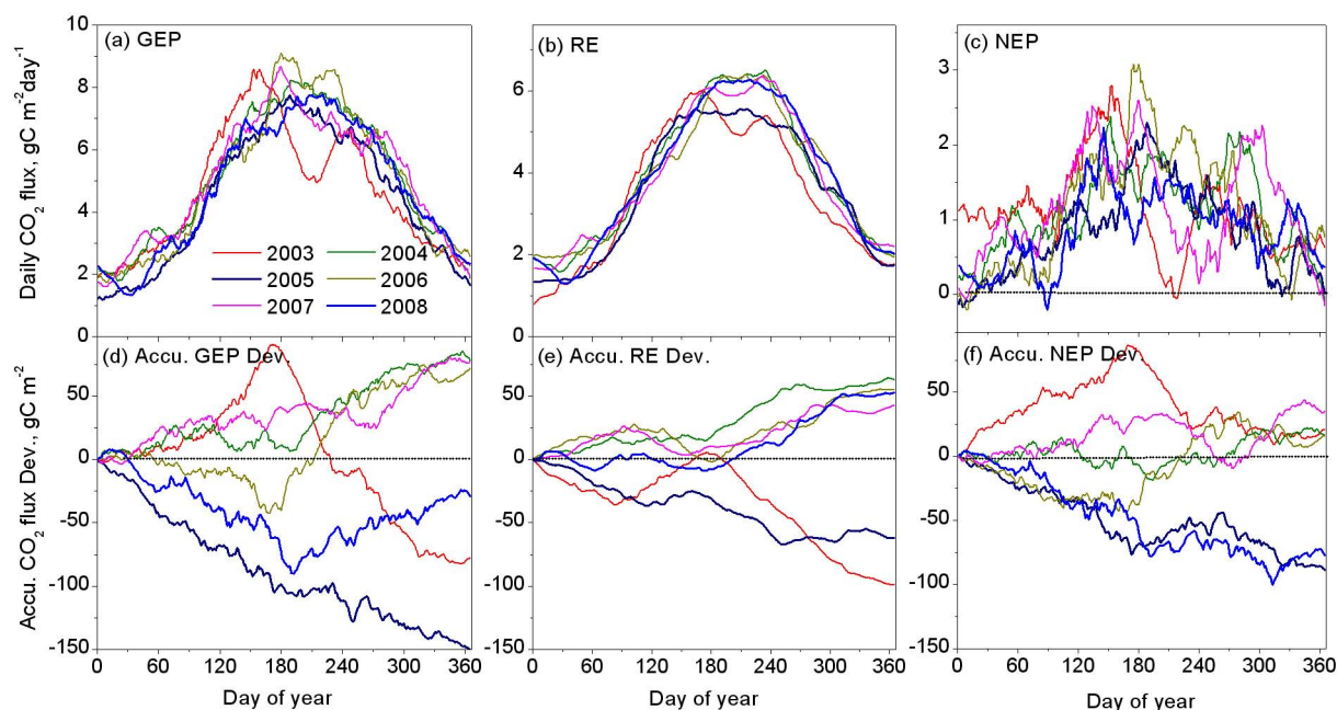
Fig. 6. The 30-day slide-averaged \text{CO}_2 fluxes (a–c) and the accumulative flux deviations (d–f) during 2003–2008. These deviation curves reflected the varying processes of \text{CO}_2 fluxes over years.
