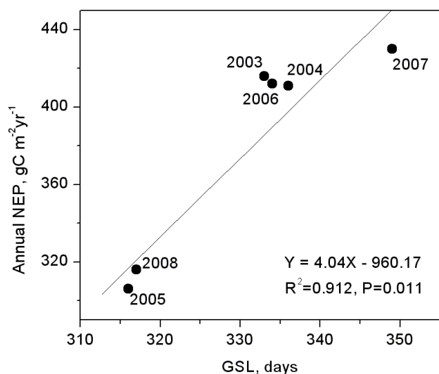
Fig. 9. Relation of annual NEP flux ( \text{gC m}^{-2} \text{yr}^{-1} ) with the growing season length ( \geq 5^\circ\text{C} , days). The line was regressed with the data of non-drought years by excluding the year 2003.
