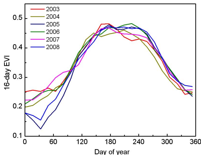
Fig. 3. Temporal curves of 16-day MODIS EVI for the coniferous plantation covered region around QYZ site. The EVI value was the average of forest pixels in this region (10 km by 10 km).
