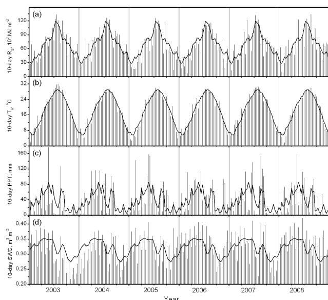
Fig. 2. The 10-day environmental conditions of QYZ site from 2003 to 2008: (a) downward solar radiation ( R_s , \times 10^3 \text{ MJ m}^{-2} ), (b) air temperature ( T_a , ^{\circ}\text{C} ), (c) precipitation (PPT, mm) and (d) soil water content (SWC, \text{m}^3 \text{ m}^{-3} ). The drop lines and curves were the 10-day measurements and corresponding multi-year averages respectively.
