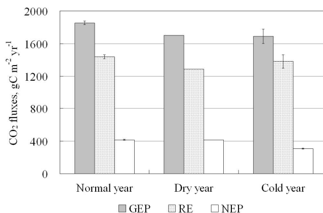
Fig. 8. Averaged annual CO 2 fluxes (g C m -2 ) of normal years (2004, 2006 and 2007), dry year (2003) and cold years (2005 and 2008) at QYZ site.
