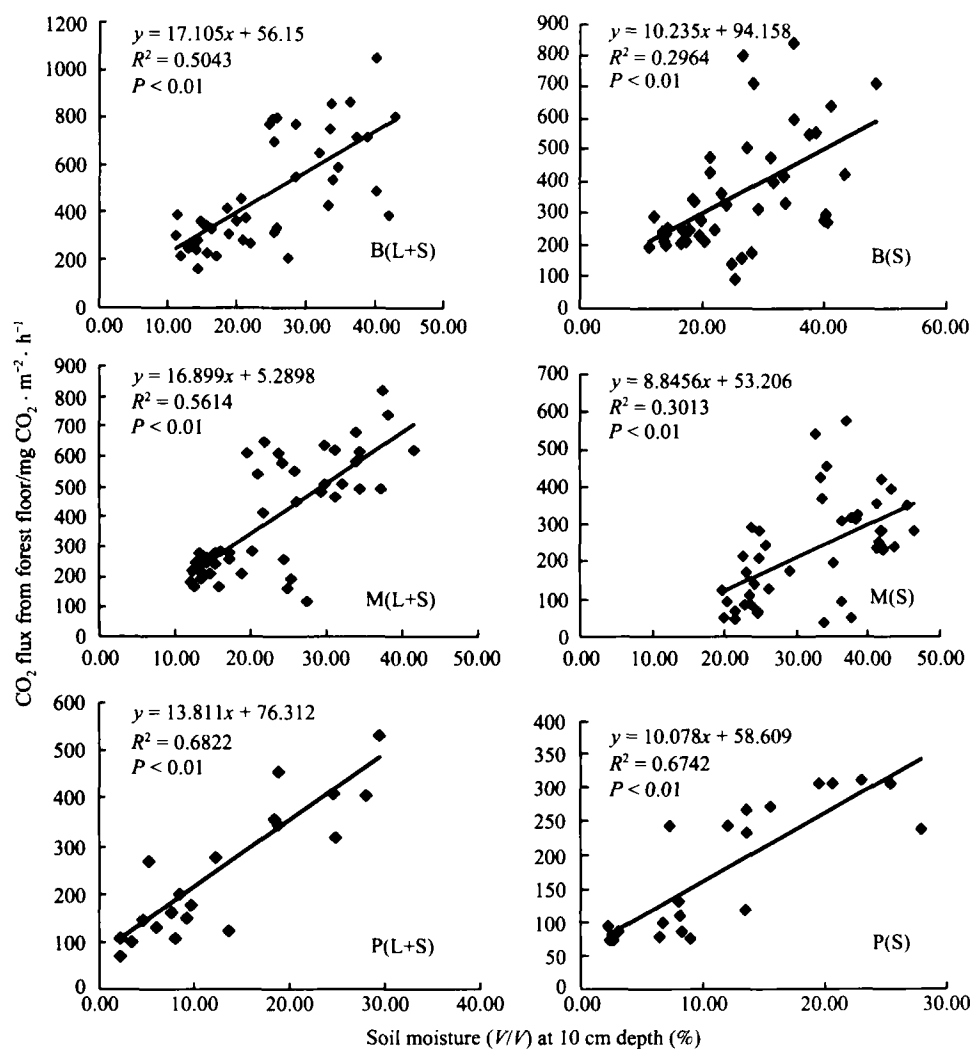
Fig. 4. Relationship between \text{CO}_2 flux and soil moisture at 10 cm depth for the three types of forest. The meanings of letters in this figure are the same as in fig. 3.
