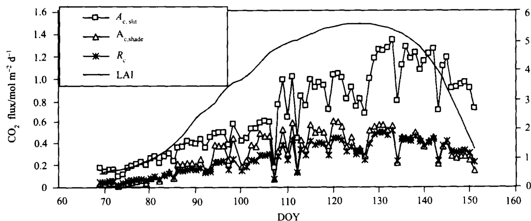
Fig. 5. Seasonal dynamics of photosynthesis rate of sunlit leaves ( A_{c,slit} ), photosynthesis rate of shaded leaves ( A_{c,shade} ), and crop respiration rate ( R_c ) with the CPCEM.
