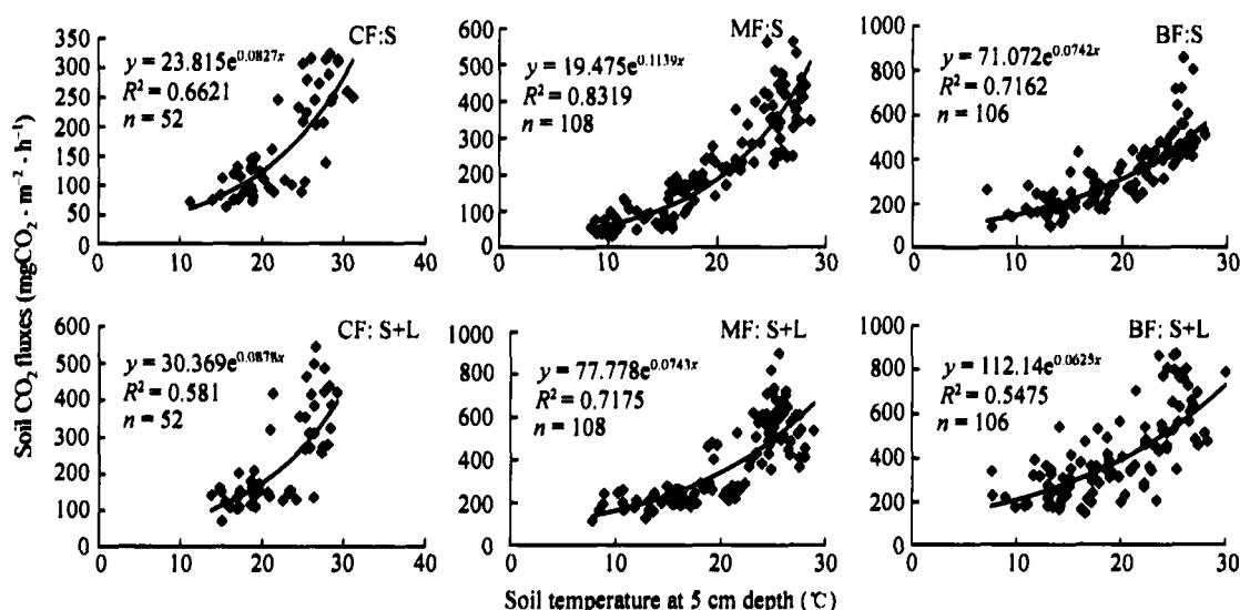
Fig. 3. The relationship between CO 2 effluxes and soil temperatures in different forests.
