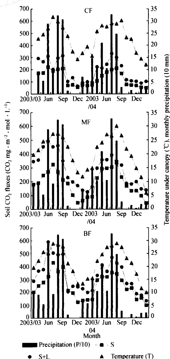
Fig. 1. Seasonal dynamics of soil CO 2 effluxes in different forests. BF, MF and CF represent monsoon broadleaf forest, mixed coniferous and broadleaf forest, and coniferous forest, respectively. The precipitation is 1:10 of the actual values.
