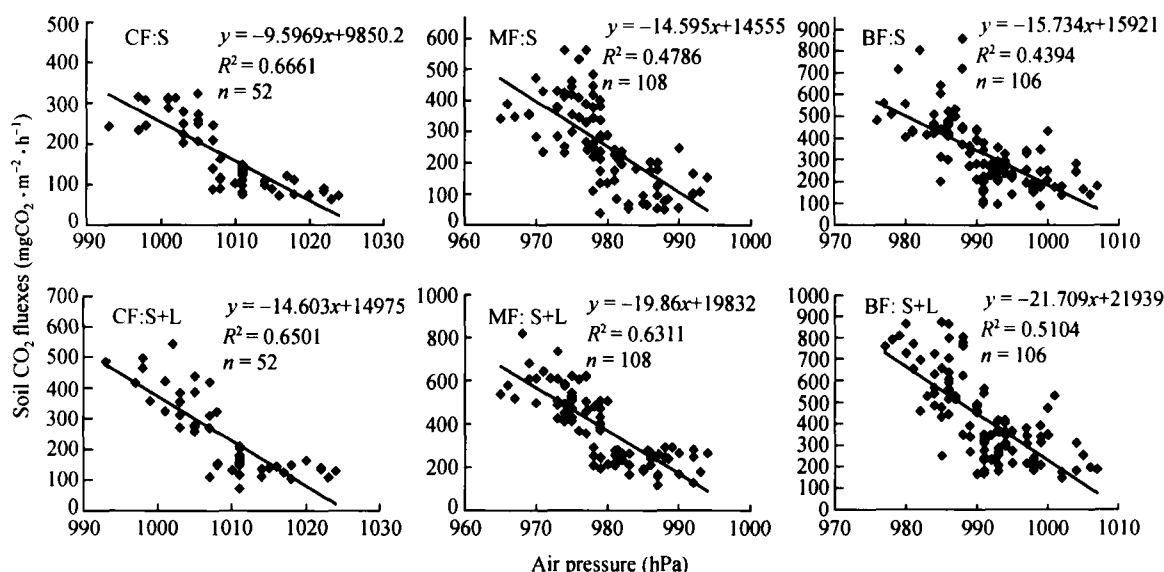
Fig. 5. The relationship between soil CO 2 efflux and atmospheric pressure.
