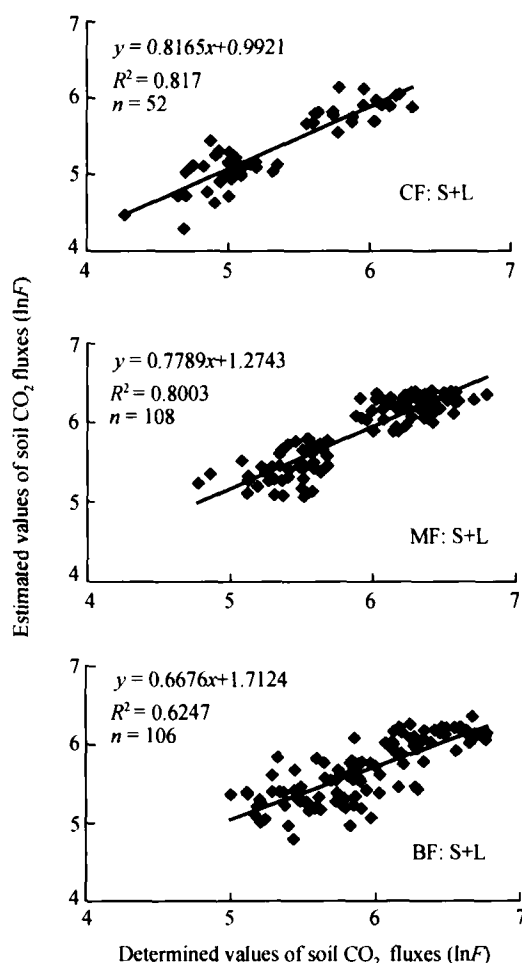
Fig. 6. Curve-fitting of forestry soil CO 2 effluxes using estimated and empirical values.
