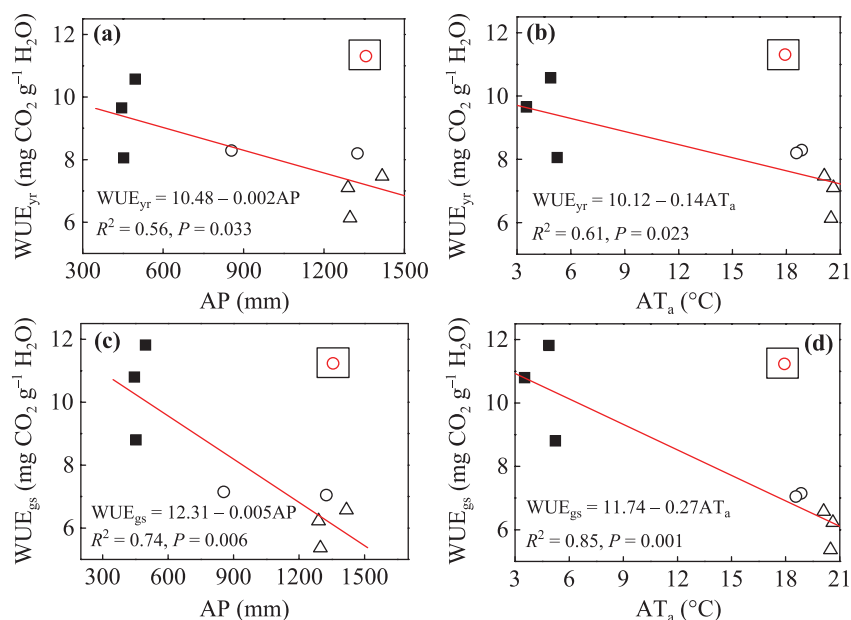
Fig. 6 The variations of vegetative season ecosystem water-use efficiency ( WUE_{gs} ) and annual ecosystem WUE ( WUE_{yr} ) with increasing annual precipitation (AP) and mean annual temperature ( AT_a ). Sites were: CBS (Changbaishan temperate broad-leaved Korean pine mixed forest, squares), QYZ (Qianyanzhou subtropical coniferous plantation, circles) and DHS (Dinghushan subtropical evergreen broad-leaved forest, triangles). The inset circle is the WUE of QYZ in 2005.
