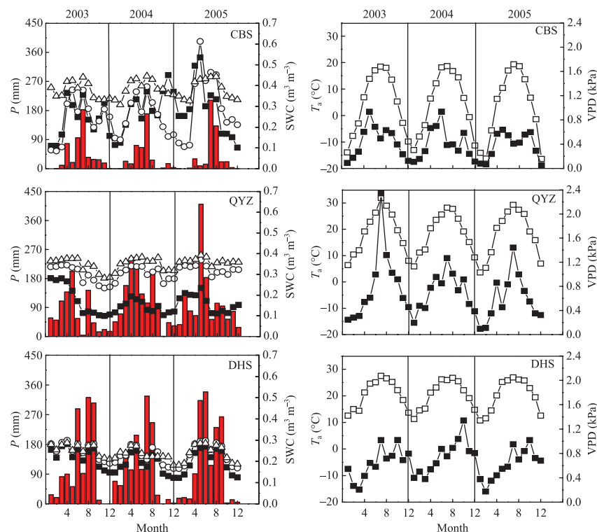
Fig. 1 The seasonal variation of precipitation ( P , columns), soil water content (SWC; closed squares, open circles and triangles are SWC at depths of 5 cm, 20 cm and 50 cm, respectively), air temperature ( T_a , open squares) and saturated vapor pressure deficit (VPD, closed squares) at CBS (Changbaishan temperate broad-leaved Korean pine mixed forest), QYZ (Qianyanzhou subtropical coniferous plantation) and DHS (Dinghushan subtropical evergreen broad-leaved forest) sites from 2003 to 2005.
